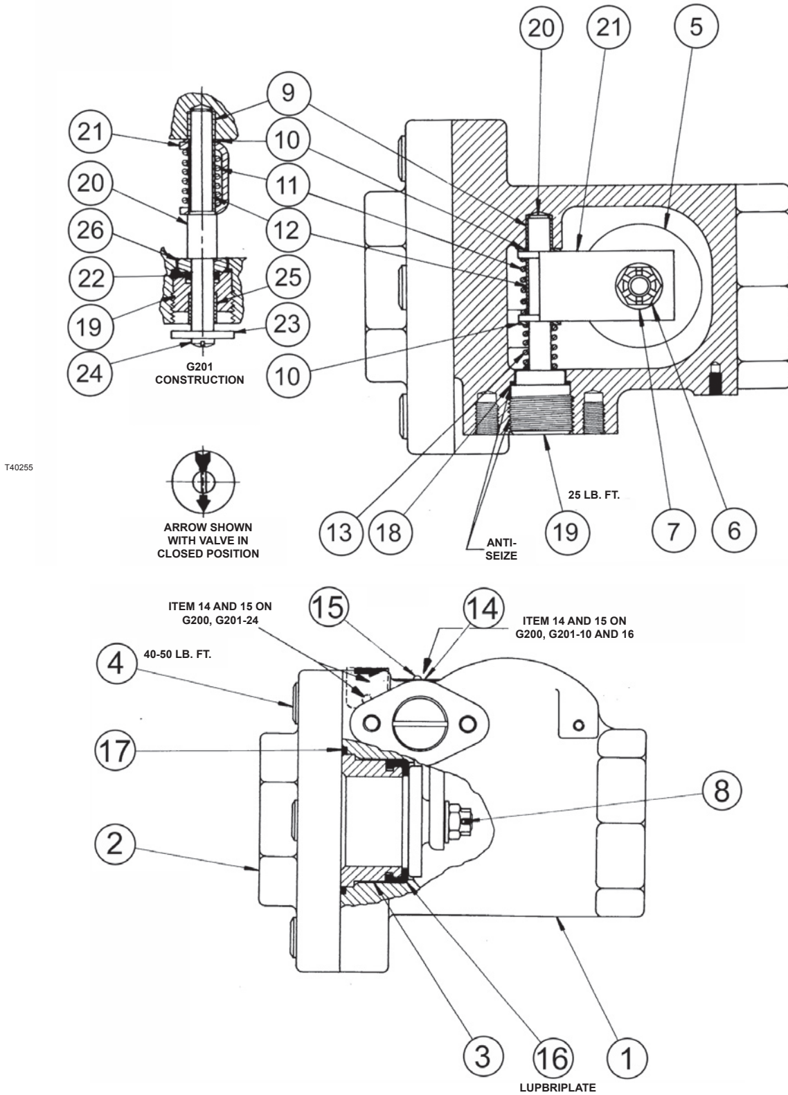
Figure 1. G200 Back Check Valve
